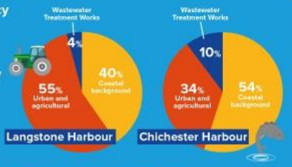
Source: Nitrate vulnerable zone designation 2017 - Eutrophic Waters, The Environment Agency
